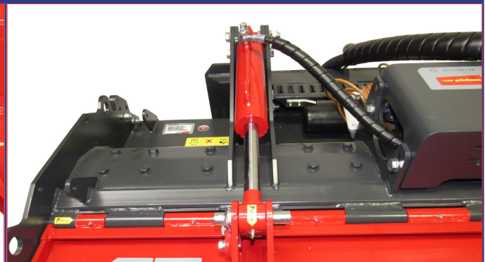
Cylinder for raising upper feed rotor/hood
